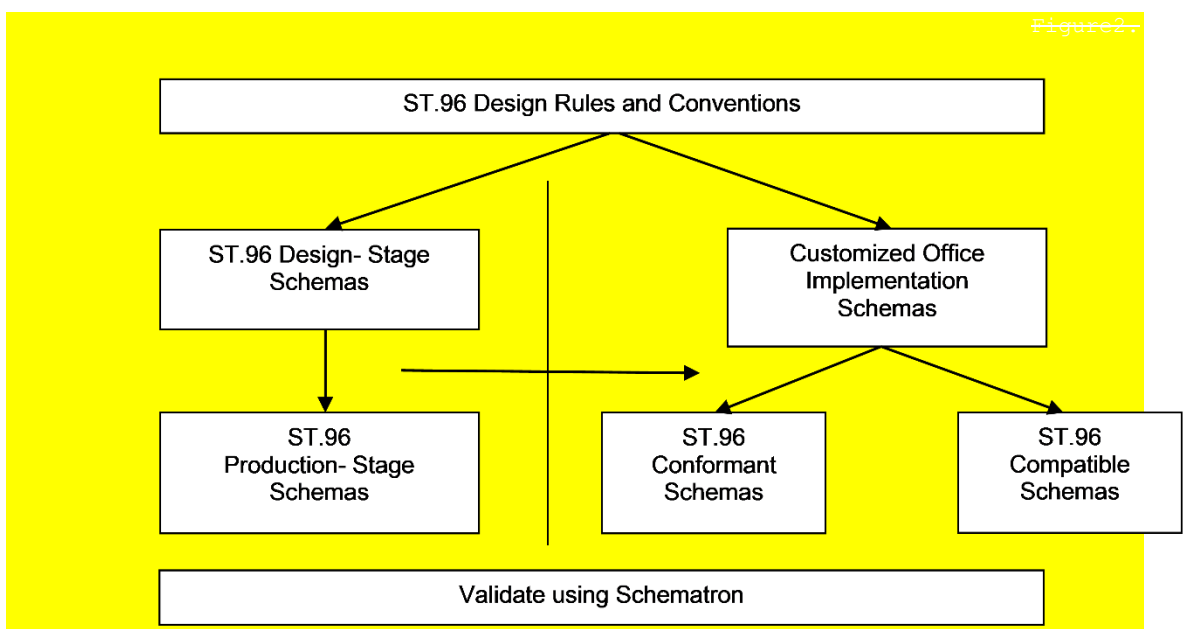
Figure 3: Overview of ST.96 customization process
