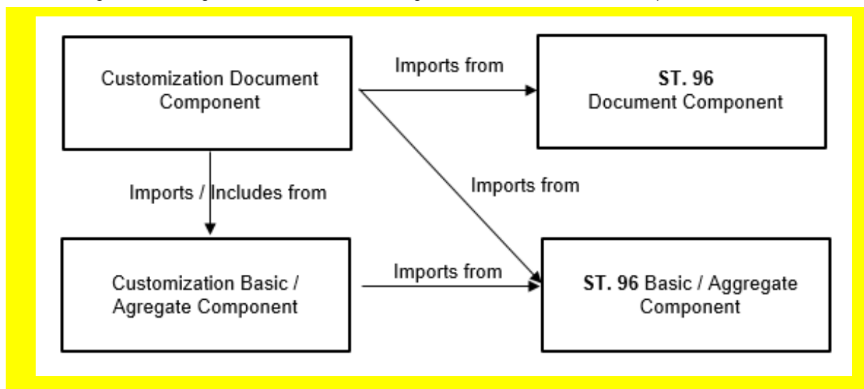
Figure 1. Using the 2: Specifying using both ST.96 Components for and non-ST.96 documents Components
