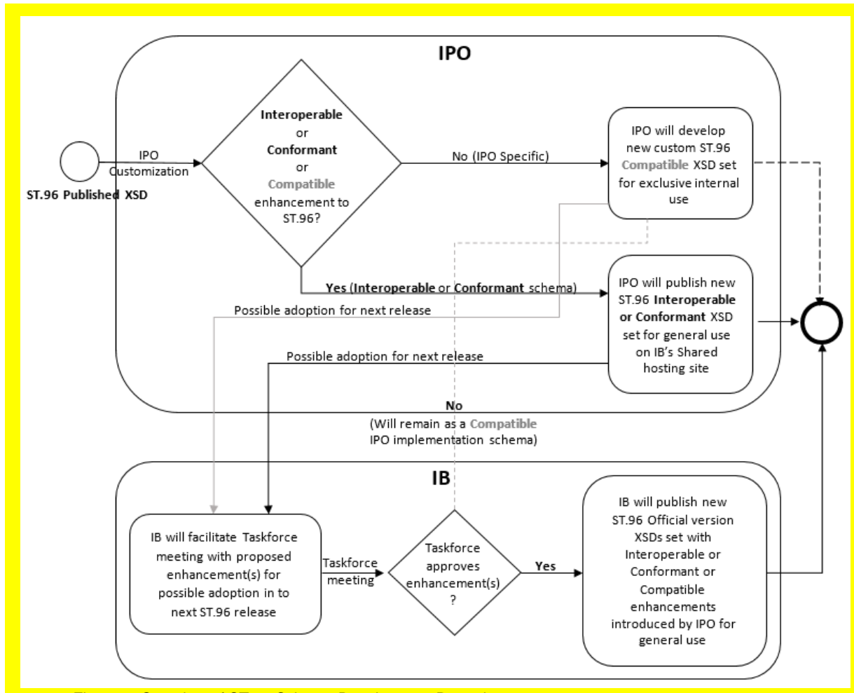
Figure 1: Overview of ST.96 Schema Development Procedure
