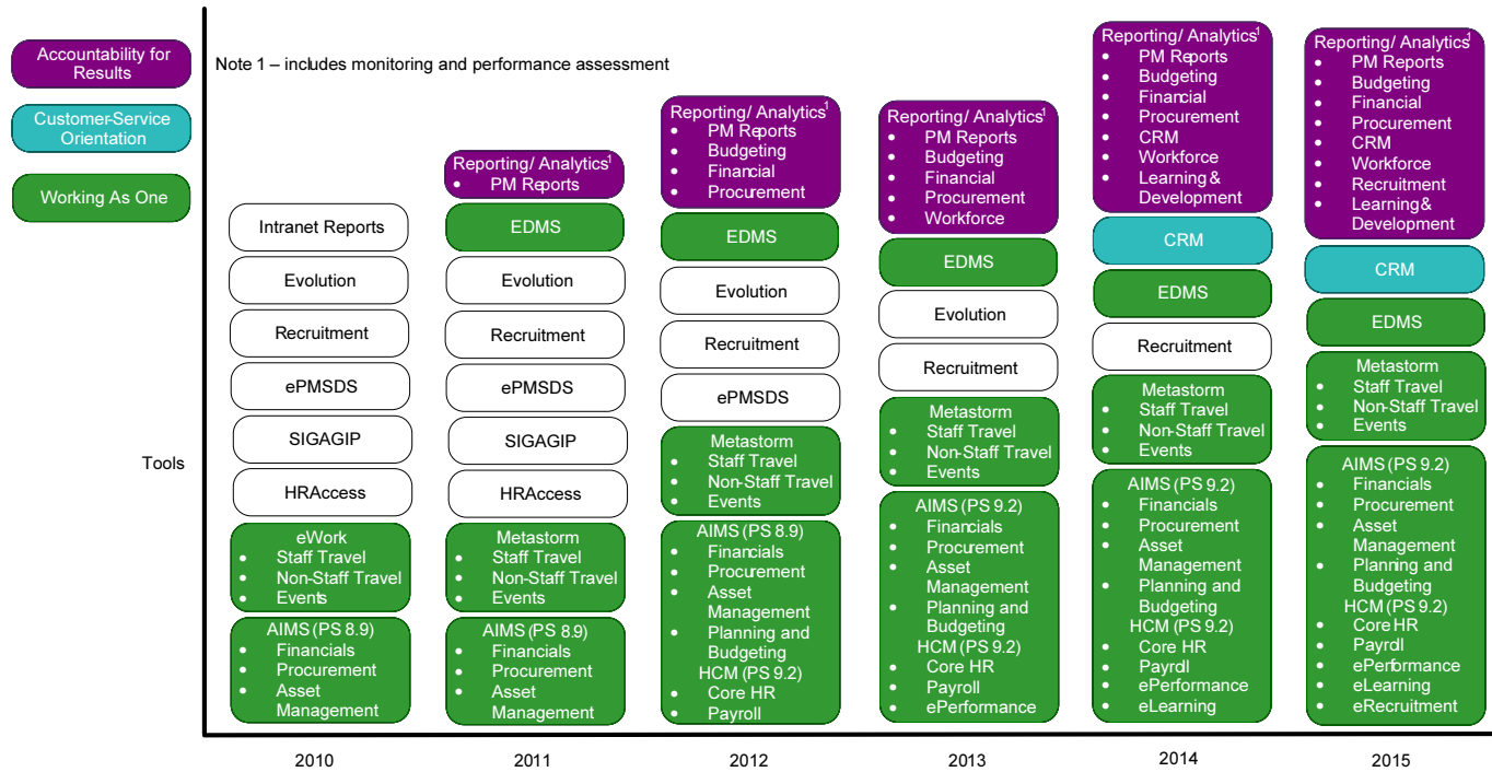
Diagram V WIPO's ERP Solution Evolution over time
