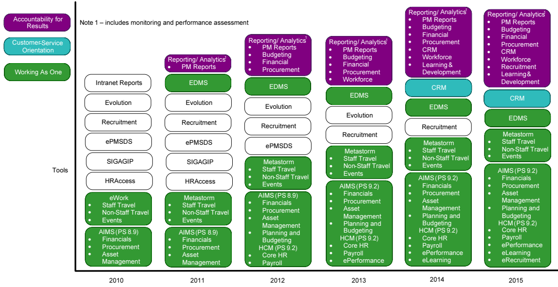
Diagram IV WIPO's ERP Solution Evolution over time
